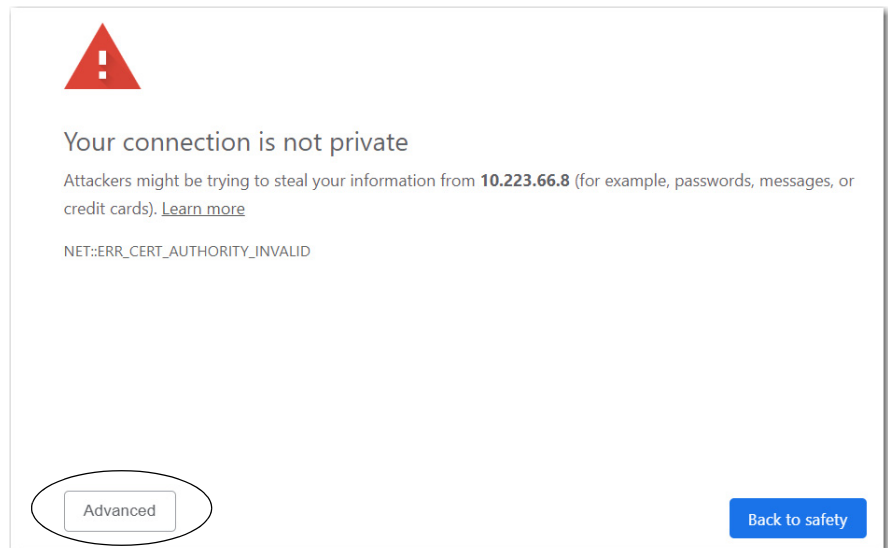
Figure 10 - Security Messages—Chrome
