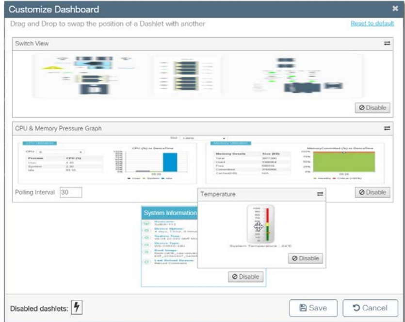
Figure 17 - Customize Dashboard
