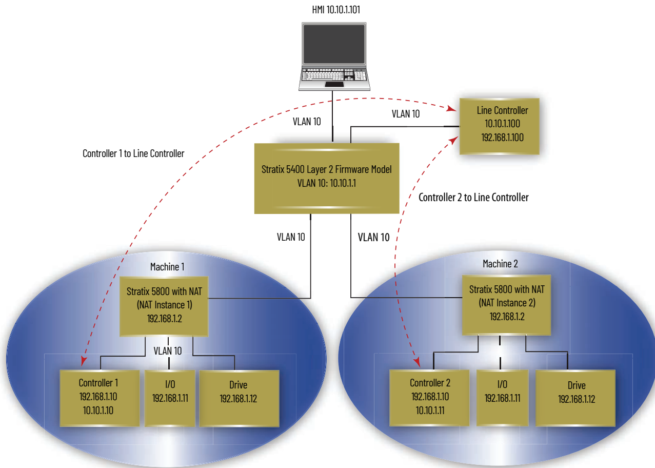
Figure 20 - Layer 2 Example with NAT in Stratix 5800 Switch
